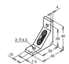
ABLR-4015-4
