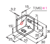
BLCM-3025-6
