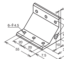
ABLH-4055-4
