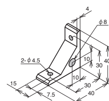
ABLH-4015-4
